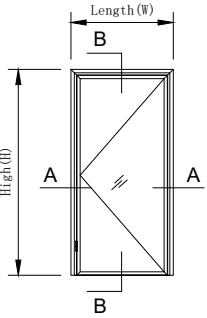
(Elevation view)
