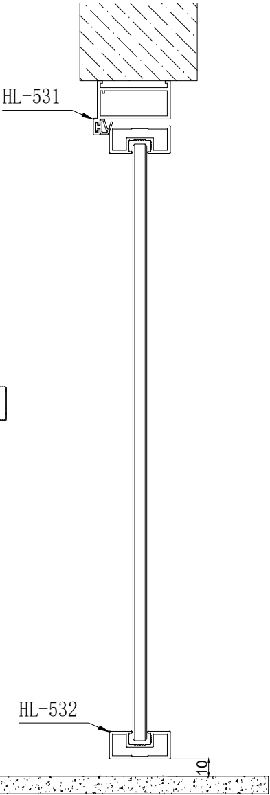
Section: B-B
